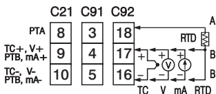
Figure 2.8 Sensor Input Wiring
