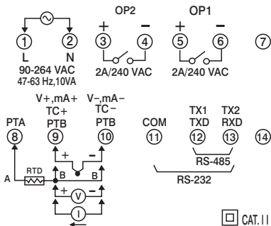
Figure 2.4 Rear Terminal Connection for C21
