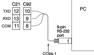
Figure 2.22 RS-232 Wiring
