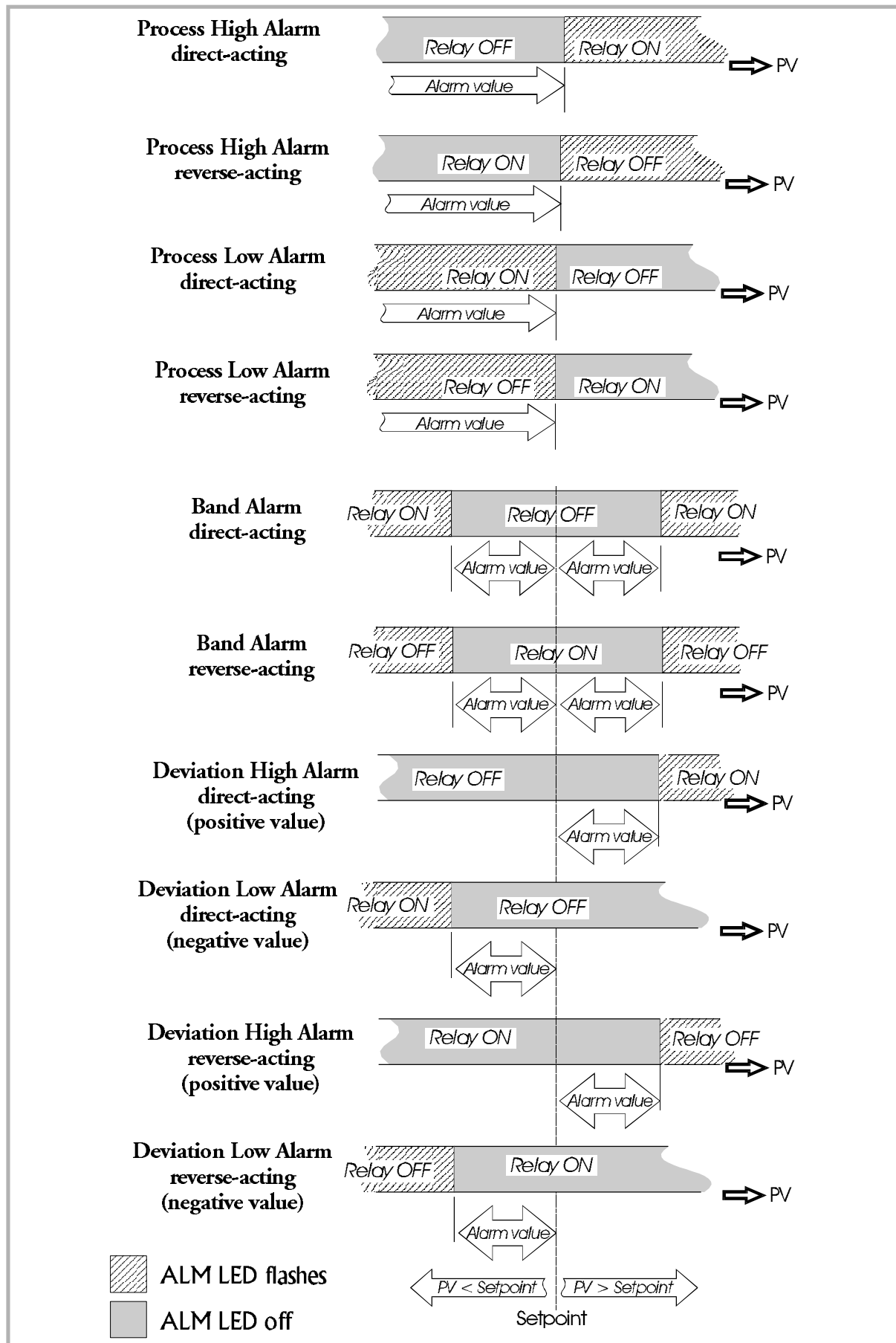
Figure 3-2 Alarm Operation
