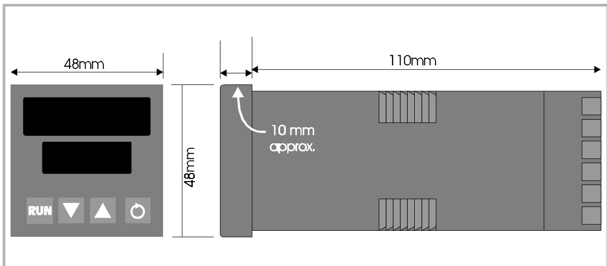
Figure 1-2 Main Dimensions
