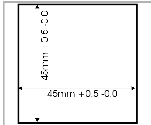
Figure 1-1 Cut-out Dimensions
